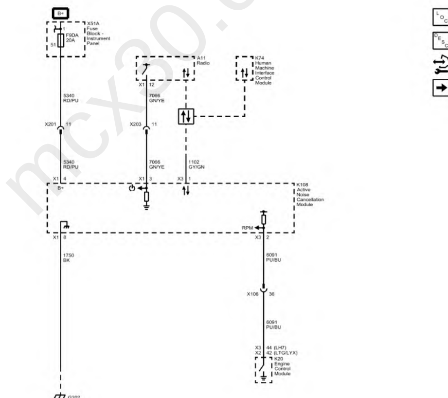
Fig. 1: Active Noise Cancellation Module Power, Ground and Serial Data (NKC with UZ6 without IOR).
